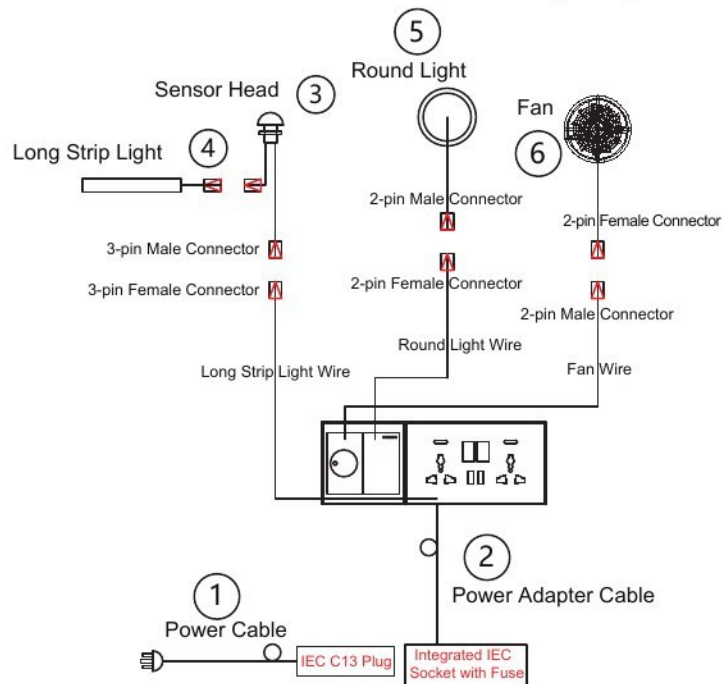
M, L, XL Multi-Person Pod Series Wiring Diagram
